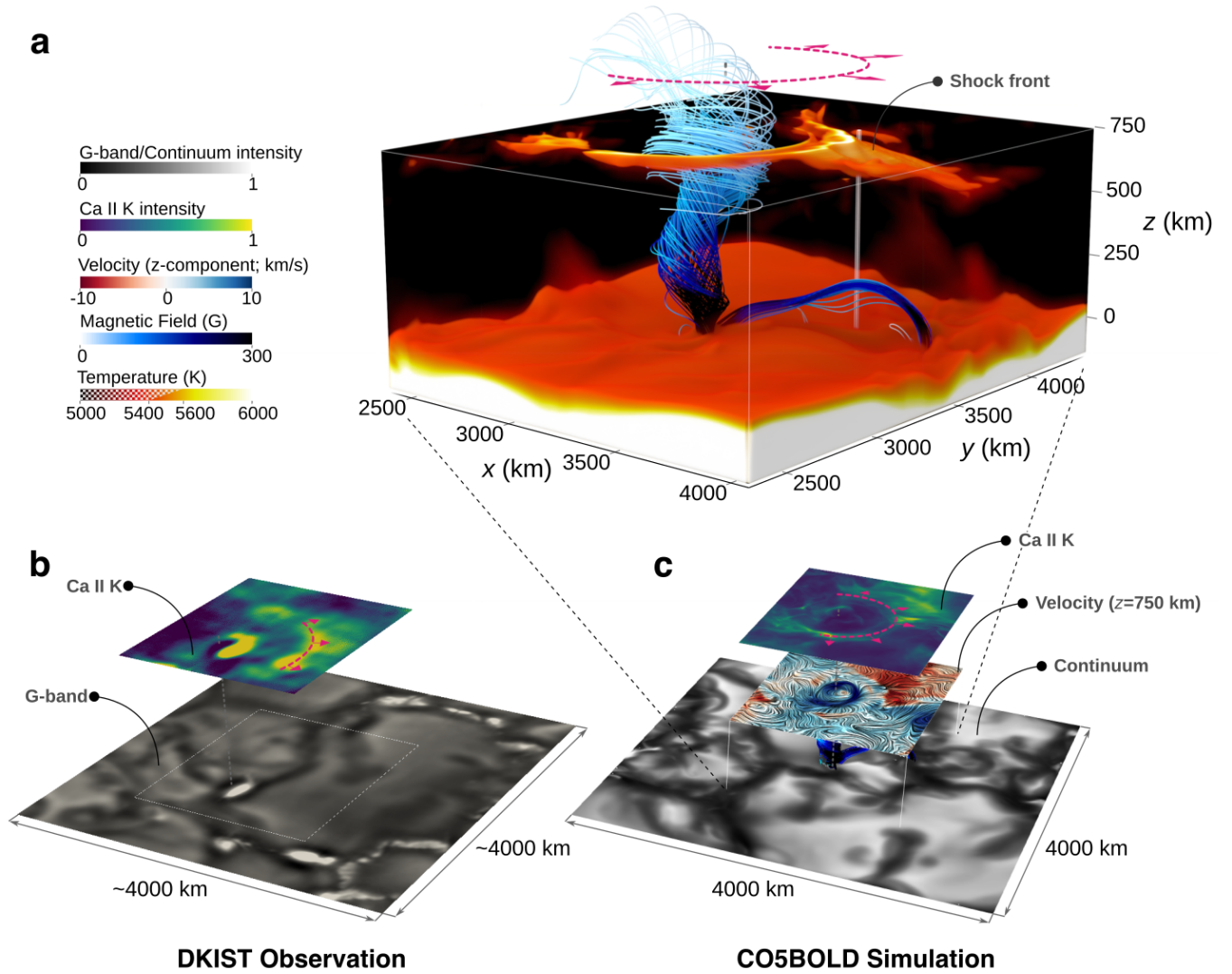
Figure 4. Comparison of the observational case Nr. E1 with a simulated atmosphere and synthesized blue continuum and Ca II K maps. (a) Volume rendering of the temperature above 5000 K of simulation event Nr. S1 (at t = 5814 s) with blue magnetic field lines representing the twisted magnetic vortex structure. The bright front appears as a thin, arc-shaped temperature enhancement on one side of the vortex illustrated by the dashed pink semicircle with arrows indicating the direction of propagation. The shock front proper is visible as the sheet of enhanced temperature slightly inclined with respect to a horizontal plane. The location of the line of sight used in Figures 7 and D2 at (x, y) = (3435 \text{ km}, 3755 \text{ km}) is shown as a white line on the right-hand side in the 3D view. (b) DKIST/VBI observations of event Nr. E1 at time t = 826 s. The pink dashed arc shown in the Ca II K image represents the location of the bright front, while arrowheads indicate the direction of travel of the front. (c) The top map shows the line-core Ca II K map referring to the low chromosphere/upper photosphere and the bottom map shows the continuum intensity at 450 nm referring to the nearly same photospheric region as the observed G-band image, both of which were computed from the numerical simulation data. The middle map displays the line integral convolution of the horizontal velocity field at z = 750 km with the colors denoting the vertical velocity, v_z , where red indicates downflows and blue indicates upflows. An animation of panel (a) is linked to this Figure. The time sequence spans a duration of 68 s and shows the evolution of the temperature and magnetic lines of force. In the time sequence, the bright front appears as a thin, arc-shaped temperature enhancement on one side of the vortex at the top boundary of the subdomain. The shock front appears as an extended sheet of enhanced temperature, slightly inclined with respect to the horizontal plane.
