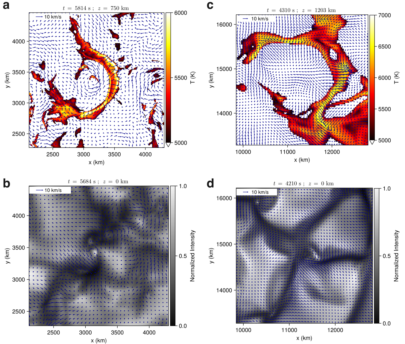
Figure 8. Horizontal velocities from the simulated atmosphere. (a) The temperature above 5000 K is shown as a background image to the horizontal velocity depicted with blue arrows for event Nr. S1 (CO5BOLD) at a height of z = 750 km at time t = 5814 s. (b) Continuum intensity at a wavelength of 450 nm as a background to the horizontal velocity for event Nr. S1 at a height of z = 0 km at time t = 5684 s. (c) The temperature above 5000 K is shown as a background image to the horizontal velocity depicted with blue arrows for event Nr. S2 (Bifrost) at a height of z = 1200 km at time t = 4310 s. (d) Continuum intensity at 450 nm as a background to the horizontal velocity for event Nr. S2 at a height of z = 0 km at time t = 4210 s.
