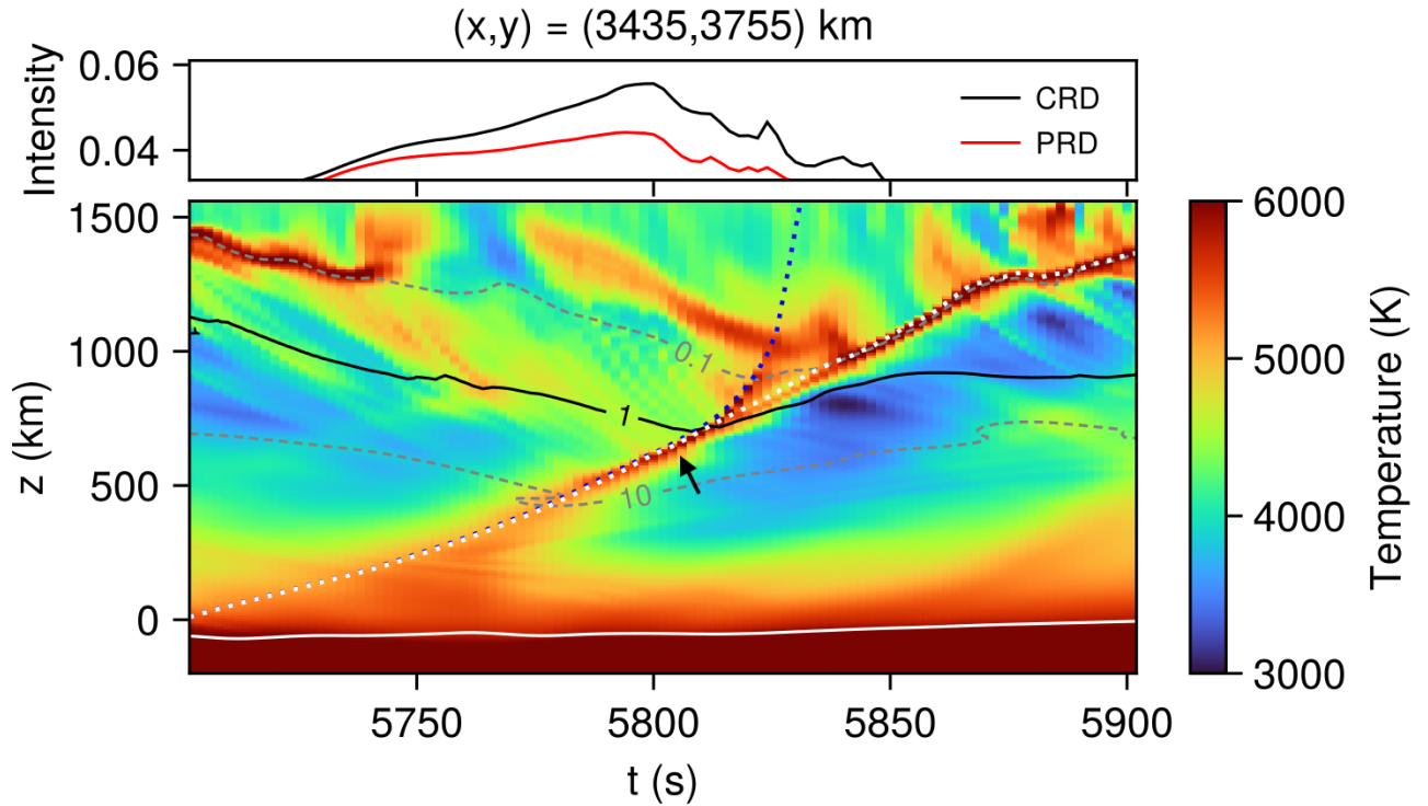
Figure 7. Time–distance diagram of the temperature from simulation event Nr. S1. The diagram shows the passage of the shock front and the corresponding variation in Ca II K filter intensity at location (x, y) = (3435 \text{ km}, 3755 \text{ km}) indicated by the vertical white line in Figure 4(a). The top panel shows the variation in the filter intensity (normalized to the intensity integrated over the full line width) calculated assuming CRD (black curve) and when taking PRD (red curve) into account. The bottom panel shows the temperature. The black arrow points at the temperature enhanced traveling shock front, which splits into two branches when crossing the \beta = 1 surface (black curve). The gray dashed contours indicate the layers of \beta = 0.1 and 10. The white line indicates the Rosseland optical depth \tau_R = 1 . The dotted paths show the trajectory of a test particle moving with the fast speed \sqrt{c_s^2 + v_a^2} plus the line-of-sight component of the velocity (blue) and the sound speed ( c_s ) plus the line-of-sight component of the velocity (white), while v_a is the Alfvén speed. Up to the branching, the two trajectories stay very close to each other because the Alfvén speed is low, and therefore the wave is a fast and predominantly acoustic wave.
