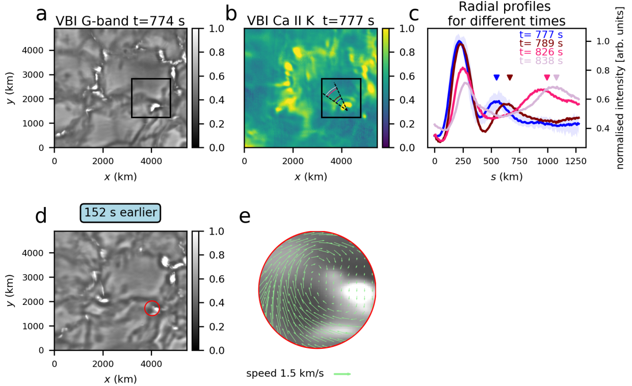
Figure 1. Wave front event Nr. E1 with the G -band BP in the photosphere, the associated Ca II K bright grain in the low chromosphere, and the emitted arc-shaped wave front. (a) Filter image of the VBI G -band channel showing the deep photosphere. The central granule is surrounded at its periphery by BP-like features, which are manifestations of small-scale magnetic flux concentrations. The BP connected to the wave phenomena discussed here is located within the black square. (b) Filter image of the VBI Ca II K channel showing the low chromosphere/upper photosphere. Within the black square, the bright chromospheric grain is partially surrounded by a bright, arc-shaped front traveling away from it. The colored arcs indicate the position of the bright front at subsequent times (see panel (c) for times). (c) Radiative intensity of the Ca II K channel (normalized to the maximum intensity of the Ca II K bright grain) along the radial direction of the travel path of the bright front. Each profile is the mean of profiles taken in 5^\circ steps between the black dashed radial lines indicated in panel (b). The shaded region around the blue curve ( t = 777 s) displays the minimum and maximum of the intensity for all curves at that time step, shown as a representative example. The position of the bright front, as inferred from the applied Gaussian fit, is marked with triangles, whereby the colors denote the time step of the observation, indicated by labels. The peak intensity at s \sim 250 km corresponds to the bright Ca II K grain from where the arc emanates. (d) G -band image recorded approximately 152 s earlier than the G -band snapshot shown in panel (b). (e) Close-up of the region of interest shown in panel (d). Green arrows display the apparent horizontal velocities obtained through a local correlation tracking method (see Section 3.1.1 for details). The velocities have been averaged over a time range of 60 s centered at the time t = 622 s. An animation of the maps of panels (a) and (b) is linked to this figure. The animation loops three times and shows a 207 s long sequence, for which the black rectangles and the dashed colored lines have been omitted. A black circle highlights the event location. A pink star indicates the location of the BP at several selected frames of the Ca II K maps and a pink dashed arc denotes the location of the bright front at times t = 771 s, t = 813 s, and t = 844 s.
