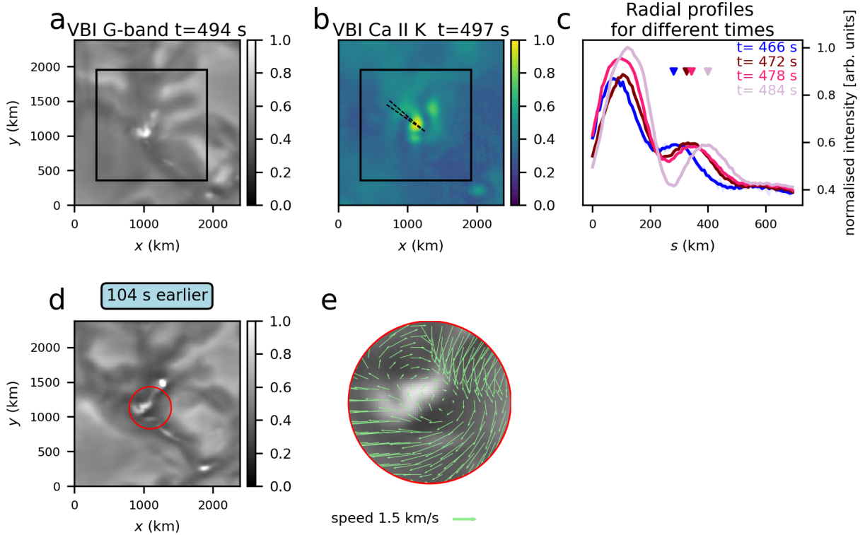
Figure 3. Event Nr. E3 of the DKIST VBI examples showing the magnetic BP located within the region of influence of a vortex in the photosphere, its corresponding signature in the low chromosphere, and the associated bright front signature. This figure is in the same format as Figure 1. For panel (e) the velocities are shown for the time t = 390 s. An animation of the images shown in panels (a) and (b) is available and linked to this figure. The animation loops three times and shows a 122 s long sequence, for which the black rectangles and the dashed colored lines have been omitted. A black circle highlights the event location. A pink star indicates the location of the BP at several selected frames of the Ca II K maps and a pink dashed arc denotes the location of the bright front at t = 503 s, t = 521 s, and t = 539 s. (An animation of this figure is available in the online article .)
