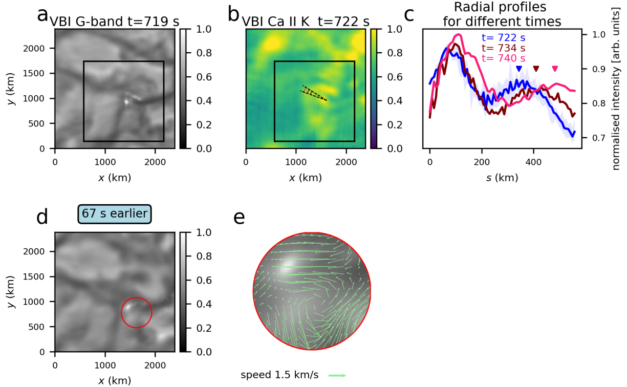
Figure 2. Event Nr. E2 of the DKIST VBI examples showing the magnetic BP located within the region of influence of a vortex in the photosphere, its corresponding signature in the low chromosphere, and the associated bright front signature. The figure is in the same format as Figure 1. For panel (e) the velocities have been averaged over a time range of 30 s centered at the time t = 646 s. An animation of the images shown in panels (a) and (b) is available and linked to this figure. The animation loops three times and shows a 140 s long sequence, for which the black rectangles and the dashed colored lines have been omitted. A black circle highlights the event location. A pink star indicates the location of the BP at several selected frames of the Ca II K maps and a pink dashed arc denotes the location of the bright front at t = 698 s, t = 716 s, and t = 734 s.
