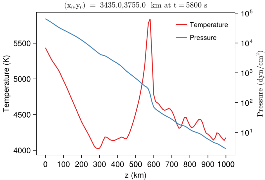
Figure D2. Temperature and gas pressure across the shock front. Temperature (red) and gas pressure (blue) along the white line of sight of Figure 4 at (x, y) = (3435 \text{ km}, 3755 \text{ km}) and time t = 5800 \text{ s} .
