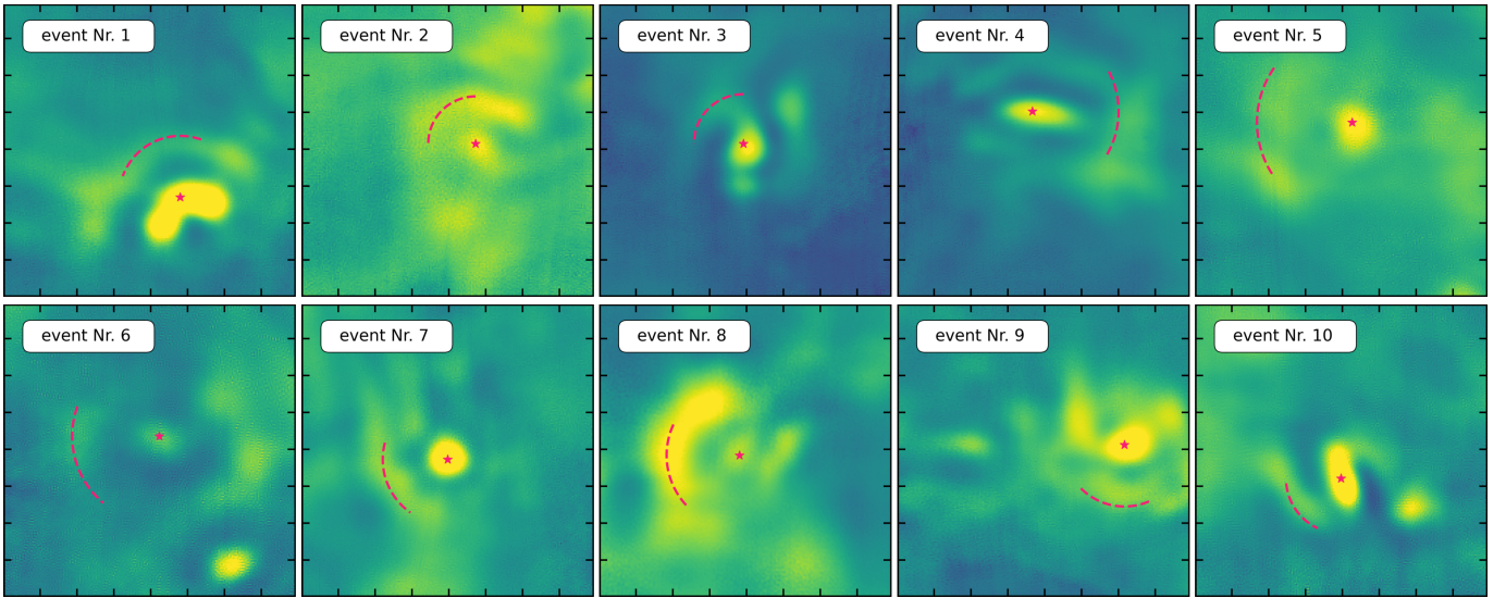
Figure B1. Collage of observed bright front events. The panels show time instances of the events seen in Ca II K with tick marks set 200 km apart. Part of the bright arc-shaped front is marked by a dashed pink arc. A pink star indicates the location of the Ca II K bright grain and corresponding G-band BPs from where the bright front emanates. An animation showing the temporal sequence of all events is linked to the present figure. The animation shows the continuum maps in the left panel and the Ca II K maps in the right panel. In the time sequence of duration 1541 s, each of the 10 events is highlighted by a colored circle during its occurrence and numbered according to the event numbers given in this figure.
