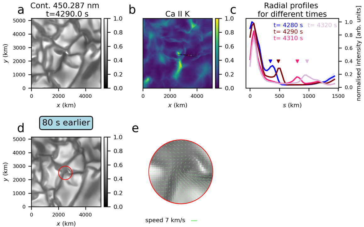
Figure 6. Simulation event Nr. S2 in the same format as Figure 1. (a) Synthesized continuum map at the wavelength 450.287 nm. The photospheric bright continuum point at (x, y) = (2300 \text{ km}, 2600 \text{ km}) is located at the source of the chromospheric arc-shaped front seen in panel (b). (b) Synthetic Ca II K map computed under CRD. The colored arcs indicate the position of the bright front at subsequent times (see panel (c) for times). (c) Normalized intensity of the Ca II K map in panel (b) along the radial direction of the travel path of the bright front. Each profile is the mean of profiles taken in 1^\circ steps between the black dashed radial lines indicated in panel (b). The position of the bright front is marked with triangles, whereby the colors denote the time step indicated by labels. The procedure to obtain these values is equivalent to the procedure used for the observational analysis. (d) Continuum image computed 80 s earlier than the Ca II K snapshot shown in panel (b). (e) Close-up of the region of interest shown in panel (d). Green arrows display the horizontal velocities extracted directly from the simulation at height z = 0 \text{ km} . For panel (e), the velocities are shown for the time t = 4210 \text{ s} . An animation of the continuum and Ca II K maps shown in panels (a) and (b) is available and linked to this figure. In the time sequence of duration 390 s, the bright arc-shaped front is marked in the Ca II K map at times t = 4290 \text{ s} and t = 4300 \text{ s} by a dashed pink arc in the replay. The pink star indicates the location of the photospheric BP during the time span of the event. (An animation of this figure is available in the online article .)
