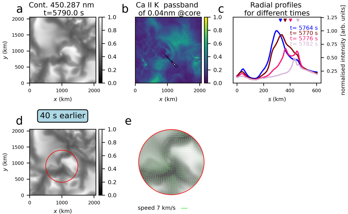
Figure 5. Simulation event Nr. S1 in the same format as Figure 1. (a) Synthesized continuum map at the wavelength 450.287 nm. The photospheric bright continuum point at (x, y) = (1000 \text{ km}, 1000 \text{ km}) is located at the source of the chromospheric arc-shaped front seen in panel (b). (b) Synthetic Ca II K map computed under PRD. The colored arcs indicate the position of the bright front at subsequent times (see panel (c) for times). (c) Normalized intensity of the Ca II K map in panel (b) along the radial direction of the travel path of the bright front. Each profile is the mean of profiles taken in 1^\circ steps between the black dashed radial lines indicated in panel (b). The position of the bright front is marked with triangles, whereby the colors denote the time step indicated by labels. The procedure to obtain these values is equivalent to the procedure used for the observational analysis. (d) Continuum image computed 40 s earlier than the Ca II K snapshot shown in panel (b). (e) Close-up of the region of interest shown in panel (d). Green arrows display the horizontal velocities extracted directly from the simulation at height z = 0 \text{ km} . For panel (e), the velocities are shown for the time t = 5750 \text{ s} . An animation of the continuum and Ca II K maps shown in panels (a) and (b) is available and linked to this figure. In the time sequence of duration 82 s, the bright arc-shaped front is marked in the Ca II K map at times t = 5800 \text{ s} , t = 5808 \text{ s} , and t = 5818 \text{ s} by a dashed pink arc in the replay. The pink star indicates the location of the photospheric BP during the time span of the event. (An animation of this figure is available in the online article .)
