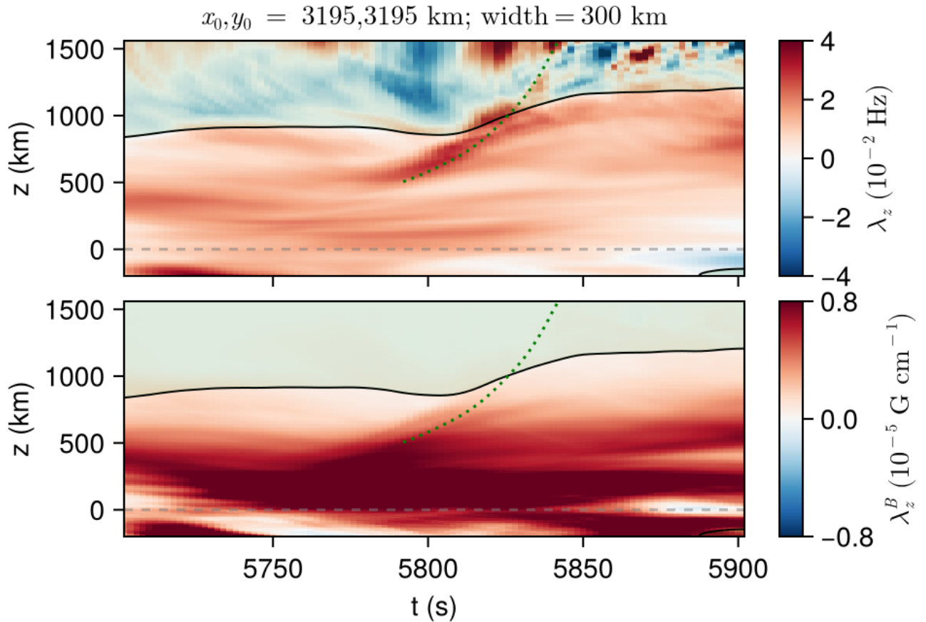
Figure 9. Time–distance diagrams of swirling strength and magnetic swirling strength. The top and bottom panels show the vertical component of the swirling vector \lambda_z , and the magnetic swirling vector \lambda_z^B , respectively, as a function of height and time for simulation event Nr. S1 shown in Figure 4. Swirling vector and magnetic swirling vector can be considered a generalization of fluid vorticity and magnetic twist, respectively (see A. F. Battaglia et al. 2021). The quantities are averaged over a horizontal area of 300 \times 300 \text{ km}^2 centered on the event at coordinates (x, y) = (3195, 3195) \text{ km} . The dotted paths show for comparison the trajectory of a test particle moving with the Alfvén speed plus vertical component of velocity. The speeds are averaged over the horizontal area. The light shaded part above the black curve shows the region where the average magnetic field is pointing upward; below it, it is pointing downwards. The ridges along the dotted curves have the same sign in \lambda_z and \lambda_z^B and move approximately with the Alfvén speed, indicative of a torsional Alfvén pulse that travels along the flux concentration with oppositely directed magnetic field. The ridges start to become visible in the top of the photosphere only where the magnetic field starts to become dynamically relevant. Also, their appearance is sensitive to the precise location of the chosen line of sight and area due to the horizontal displacement of the vortex and magnetic field with time.
