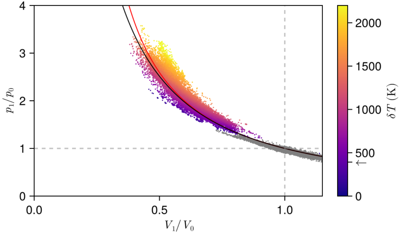
Figure D1. Pressure–volume ( p – V ) diagram showing the shocked and the quiescent condition. The temperature difference between pre- and postshock medium is displayed. The quiescent conditions (gray dots) follow the isentropic curve with minor volume compression and expansion typical of an acoustic disturbance. The temperature variations in the quiescent conditions are less than 392 K (marked by an arrow in the colorbar). The shocked state (colored dots) still essentially follows the isentropic curve but shows larger temperature changes with compression and pressure enhancements. Yet, plasma speeds relative to the shock front stay close to sonic, indicative of a weak shock. For comparison, the red and black curves show the Hugoniot and isentropic tracks, respectively, for a constant, mean \gamma = 1.33 .
