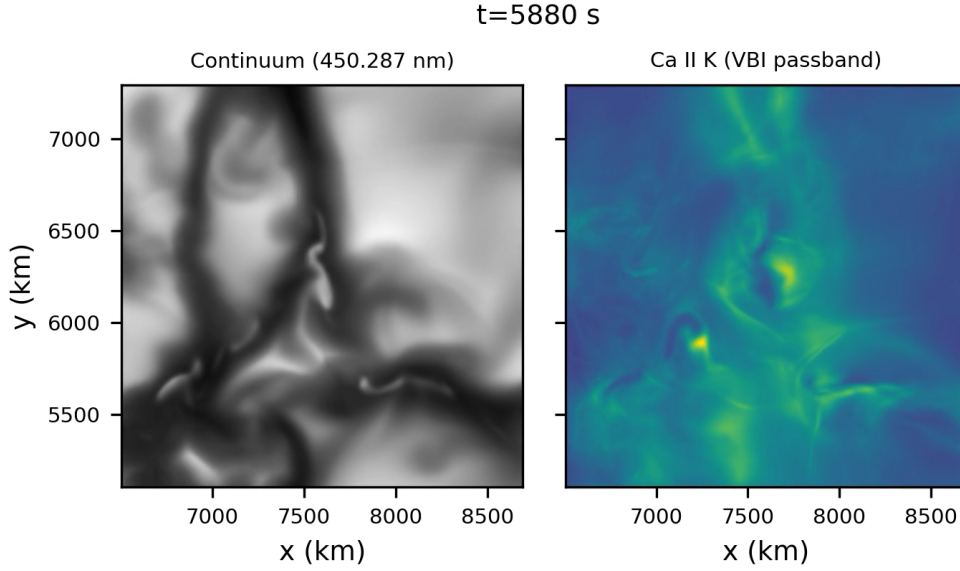
Figure C1. Synthesized maps from simulation event Nr. S3: The animation shows in the right panel the synthesized Ca II K passband filter maps referring to the low chromosphere/upper photosphere and the left panel maps of the continuum intensity at 450 nm as a close proxy for the observational G -band images, both computed from the CO5BOLD numerical simulation. The time sequence of duration 102 s shows the bright arc-shaped front marked in the Ca II K map at times t = 5896 s, t = 5904 s, and t = 5912 s by a dashed pink arc in the replay. The pink star indicates the location of the photospheric BP during the time span of the event. (An animation of this figure is available in the online article .)
