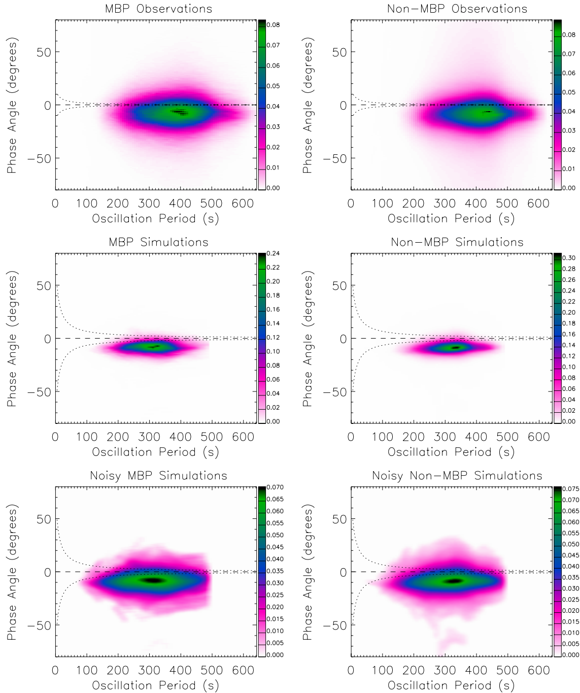
Figure 4. Occurrence of oscillations simultaneously visible in both G -band and 4170 \text{ \AA} continuum images, as a function of oscillation period and phase angle for MBP (left) and non-MBP (right) regions. The upper panels represent oscillations occurring in the observational time series, while the middle and lower panels display oscillatory phenomena detected in the noise-free and 5% added noise simulated data sets, respectively. The color scale represents the number of detections as a percentage of the total events with an associated coherence level exceeding 0.85. Consequently, the sum of each panel equals 100%. Dotted lines highlight a region inside which detections become unreliable due to cadence restrictions (0.528 s and 2 s for observational and simulated time series, respectively), while a horizontal dashed line represents a phase angle of 0^\circ . A negative phase shift implies that an oscillation detected in the 4170 \text{ \AA} continuum leads one also detected in the G band. (A color version of this figure is available in the online journal.)
